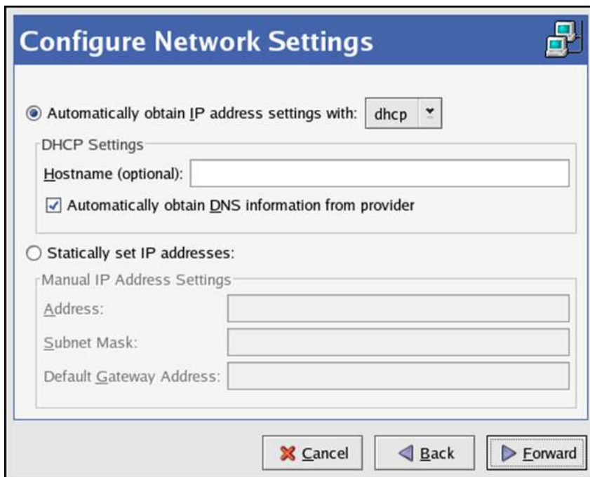
Figure 11 - Network Configuration Dialog Box
