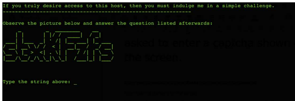
Figure 2 – Captcha Screen
