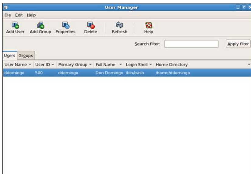
Figure 7- User Manager
