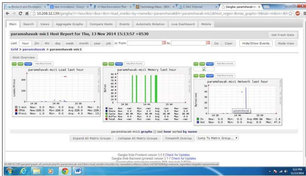
Figure 17 - ParamShavak-mic1 graphs last hour sorted by name
