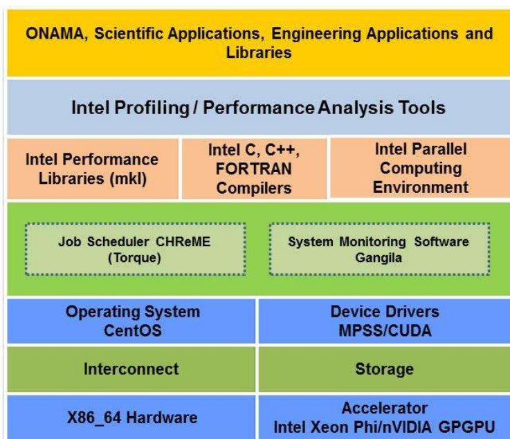
Figure 1 - PARAM Shavak Software Architecture Block Diagram
